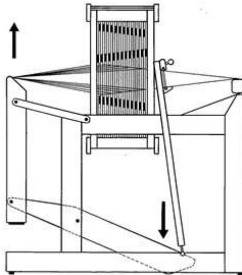
Progressive shed achieved during treadingling
